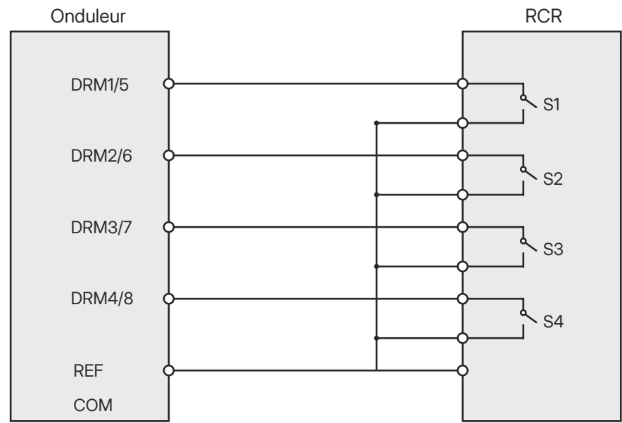
Figure 7-5 Connexion RCR
