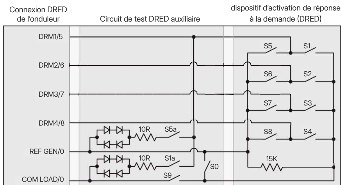
Figure 7-4 Connexion DRED
